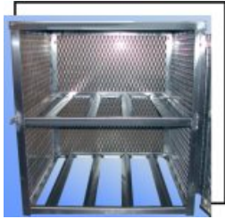
Interior racking system for horizontal cylinder storage
