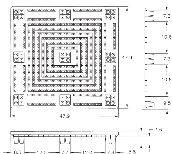
Nestable 48 x 48 C1SF Pallet
