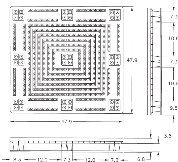
Stackable 48 x 48 C1SF Pallet
