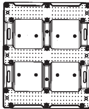
Stringer design with optional grommets
