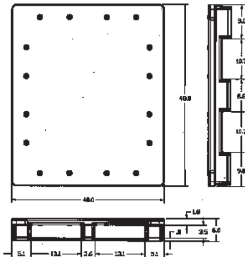
Pallet deck with optional grommets
